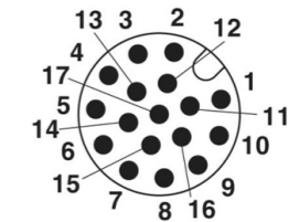
M12 17-pole male Power, COM, and I/O connector
